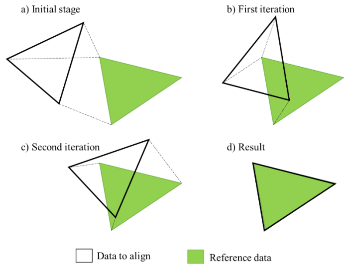
Fig. 6. Scheme of operation of the ICP algorithm in 2D data.
